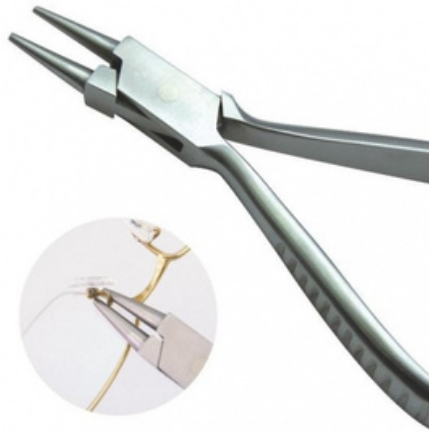
Round Snipe Nose Pliers AI-01-126 General use to adjust bridges, nose pads and joints. Intended to bend very small curves. Length: approx. 150 mm Jaws Tip: Diameter 1.2 mm Weight: approx. 117 g
